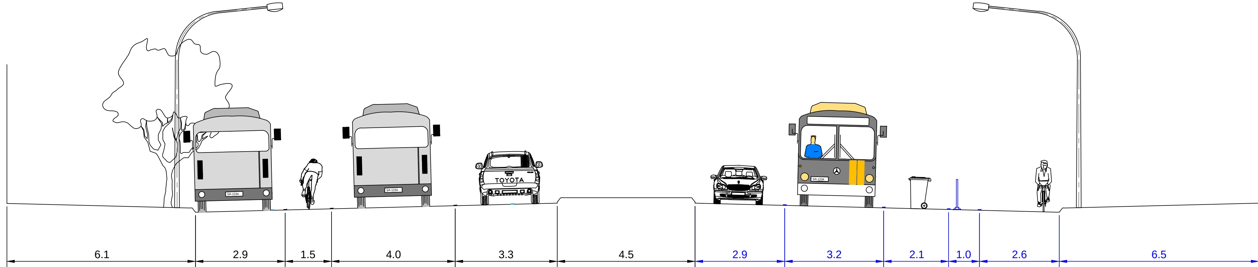
Section 2 1:75
