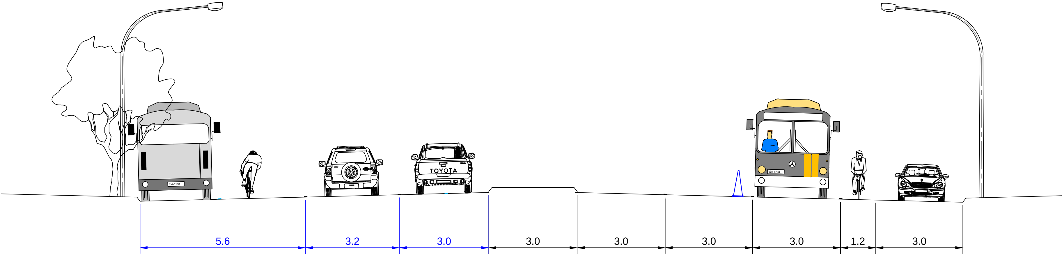
Section 1 1:75
